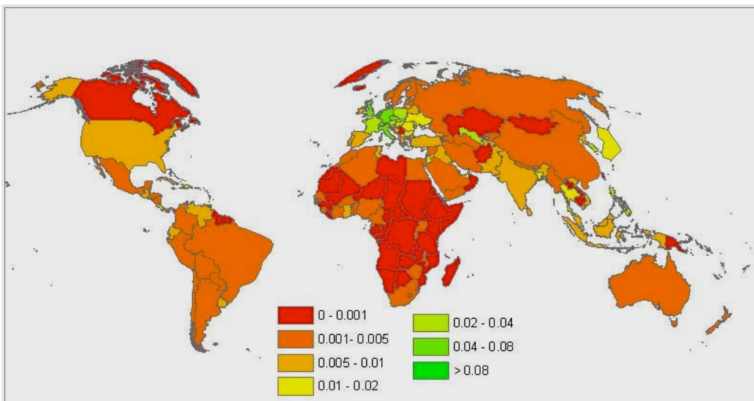
Figure 4.5: Urban land cover as a share of total land area in all countries, 2000
