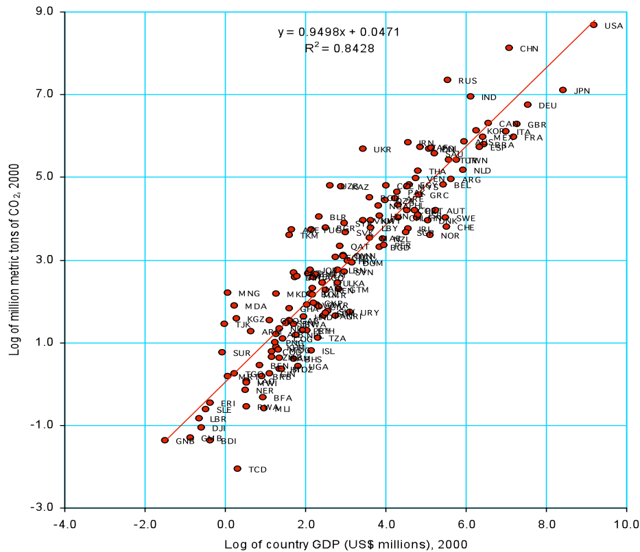
Figure 7.1: CO 2 Emissions as a function of country GDP (in log form), 2000
