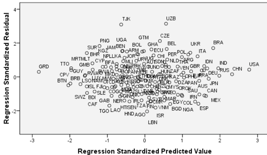
Figure 5.3: Scatter Diagram for Model 5, with Country Urban Land Cover in 2000 as a Dependent Variable
