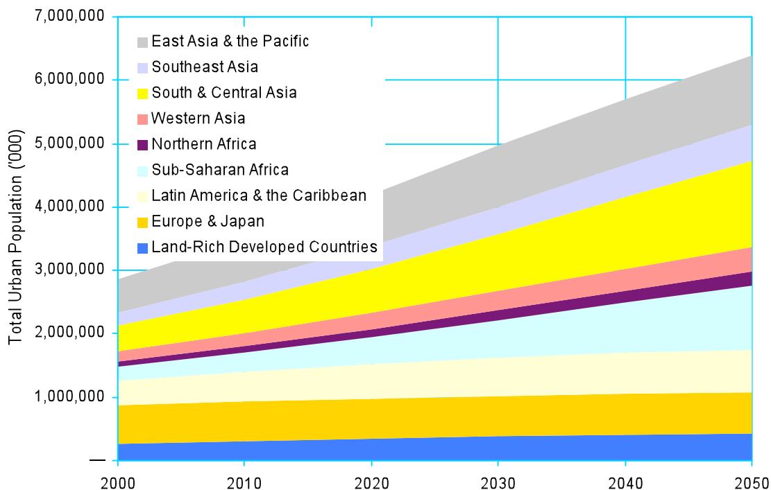
Figure 6.2: Urban Population Projections for Different World Regions, 2000-2050
