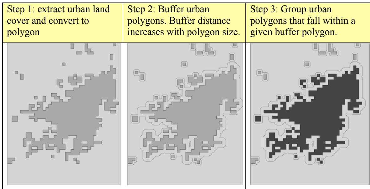
Figure 2.6: The procedure for creating urban clusters from the MOD500 land cover map
