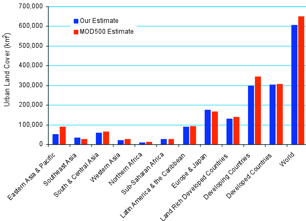
Figure 4.1: A Comparison of our estimates of urban land cover and the MOD500 map estimates for all regions, 2000
