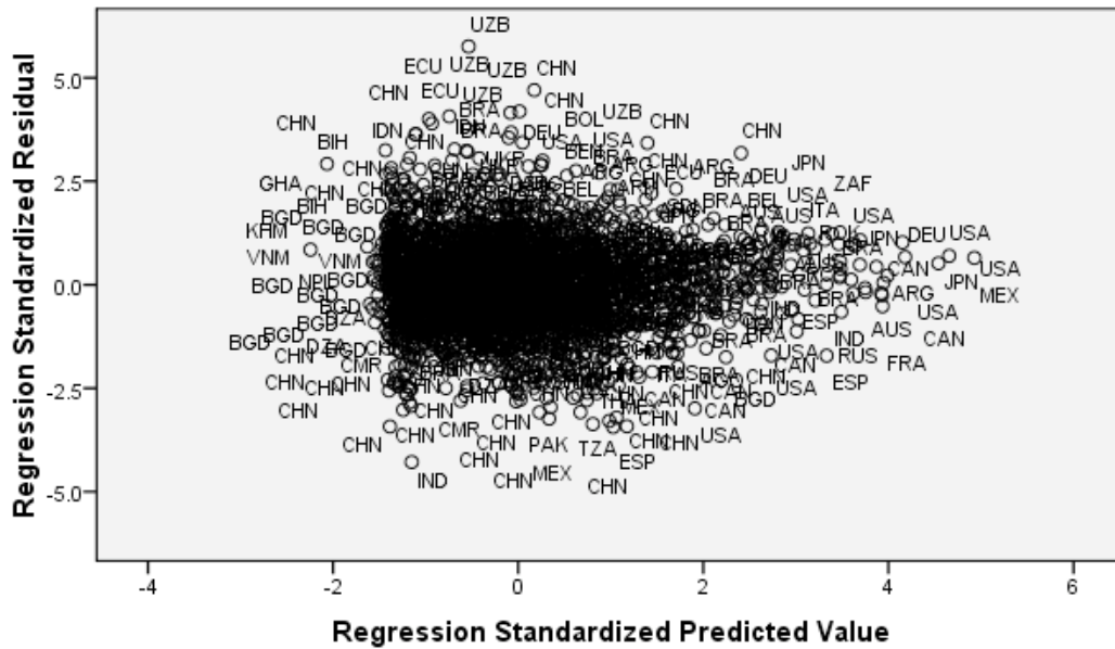
Figure 5.5: Scatter Diagram for Model 4, with Land Cover in Individual Large Cities in 2000 as a Dependent Variable
