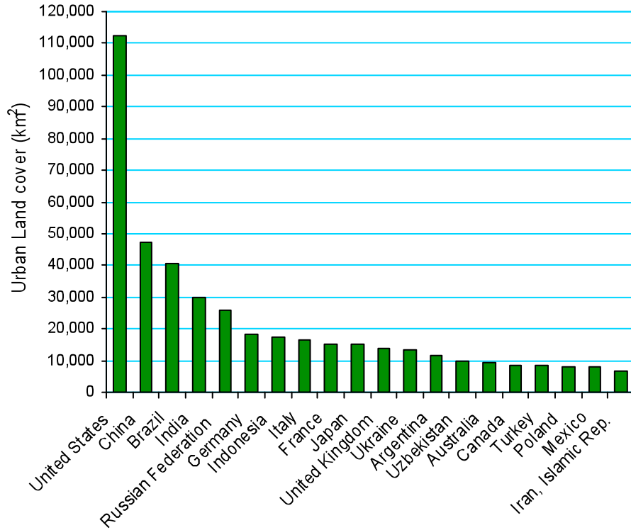
Figure 4.2: The 20 Countries with the highest areas of urban land cover, 2000
