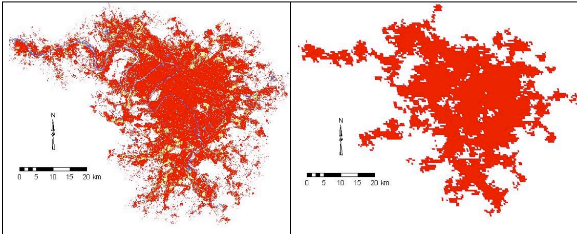
Figure 2.3: Landsat-based (left) and MOD500-based (right) urban land cover in Paris, 2000
