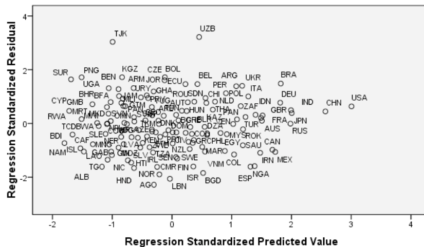
Figure 5.4: Scatter Diagram for Model 5, with Total Land Cover in Large Cities in Each Country in 2000 as a Dependent Variable
