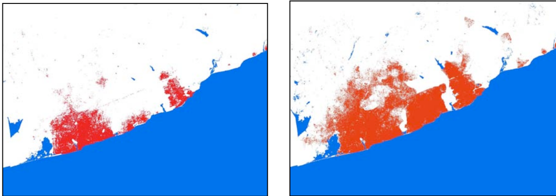
Figure 1.1: The expansion of the built-up area of Accra, Ghana (shown in red), 1985-2000
