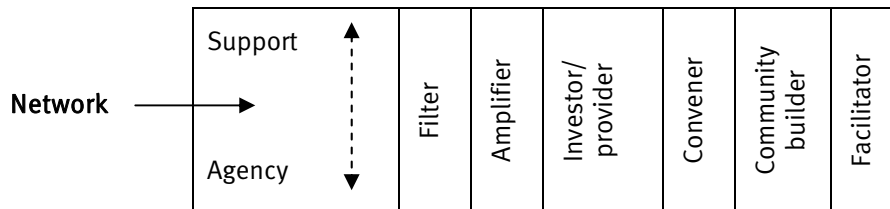
Figure 3: Describing networks
